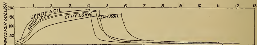
FIG. 2.—Solution curves. Absorption of phosphate by soils from a solution of monocalcium phosphate and the removal of the absorbed phosphate by water.
